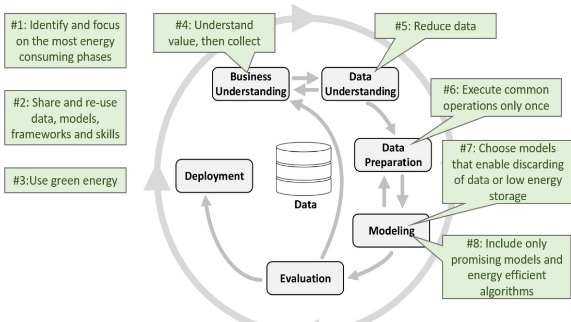
Figure 1: Crisp DM with “green” design principles
